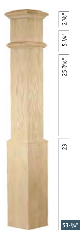
C-4090 Plain Base Width 6-1/4" RO, POP, PRM, HM, WO
