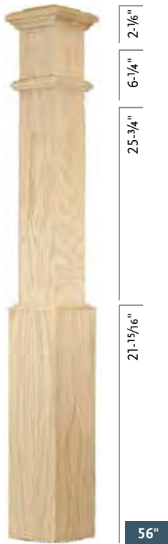
C-4891 Plain Base Width 7-1/2" RO, POP, PRM, HM, WO
