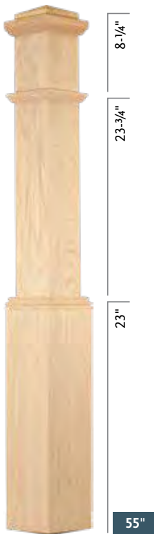
C-4091 Plain Base Width 6-1/4" RO, BEE, POP, PRM, HM, WO (RO, POP, and PR do not include EZ Mount Block)
